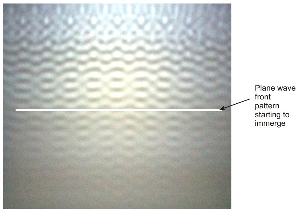
Diagram 44: Multi-point source wave front. Compare this to the double point wave pattern and notice how the waves and getting closer to looking like a plane wave.
