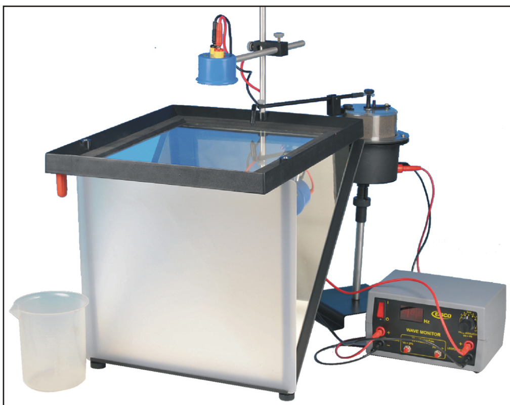
Diagram 15: Complete set up of apparatus, including a catch bucket.
